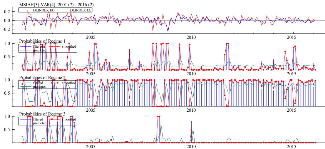
Figure 4: Regime Probabilities
